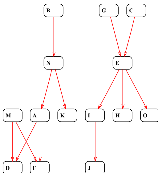
Figure 1. Graphe implicatif.
